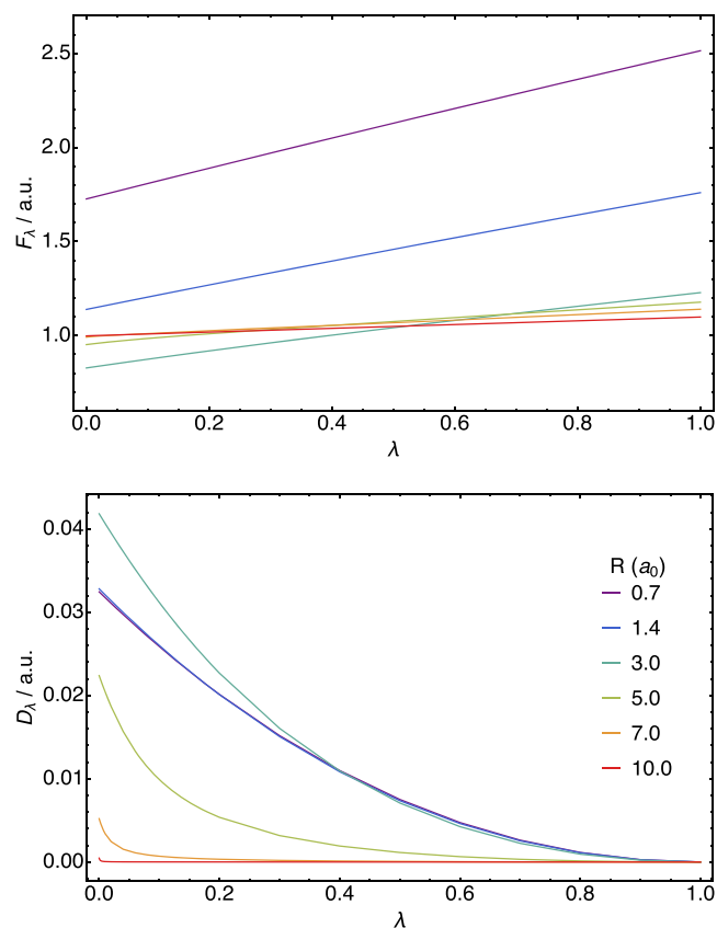
FIG. 1. F_\lambda of Eq. (9), upper panel, and D_\lambda of Eq. (31), lower panel (a.u.) as functions of the interaction strength \lambda for the \text{H}_2 molecule at internuclear separations R = 0.7, 1.4, 3.0, 5.0, 7.0, and 10.0 a.u.
